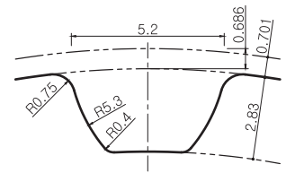
Tooth Profile: S8M / Pitch: 8mm
