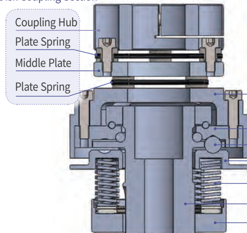
Disk Coupling Section
