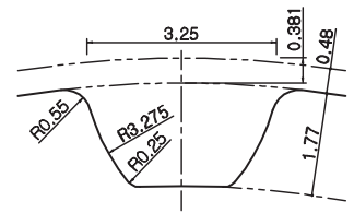
Tooth Profile: S5M / Pitch: 5mm
