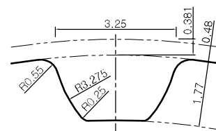
歯型:S5M / Pitch:5mm
