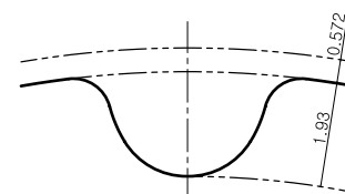
歯型:5GT / Pitch:5mm
