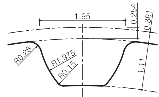
치형: S3M / Pitch: 3mm
