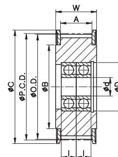
IDTC TYPE (더블베어링)
